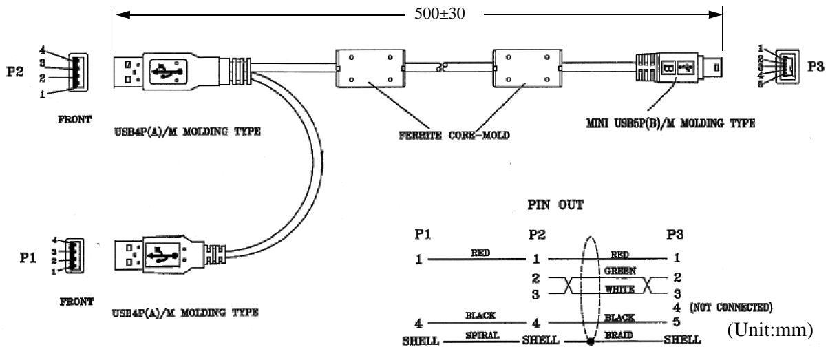
(Fig. 2-1) USB Cable
